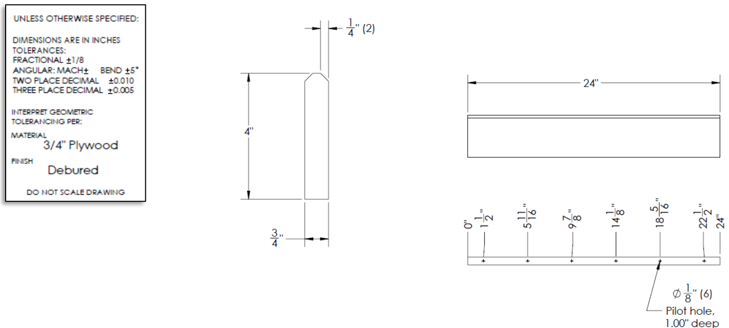
Figure 1: Cryptobox Main Fin Cut Diagram
