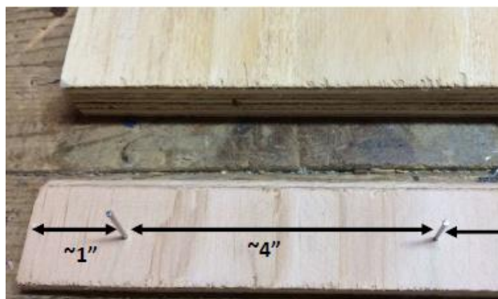
Figure 31: Partially nail in (6) nails on the chamfer side of the Cryptobox Side fins.
