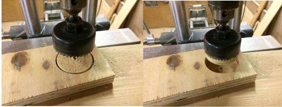
Figure 17: Use a 2 1/4" hole saw to cut out Jewel Holder holes.
