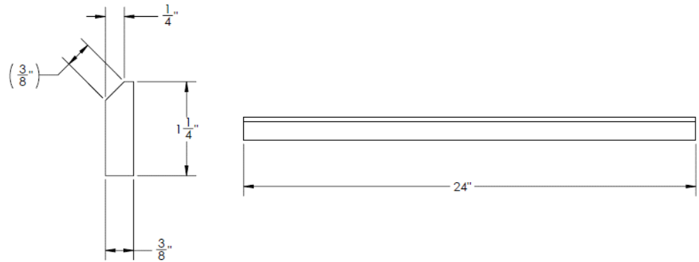
Figure 20: Cryptobox Side Fin Cut Diagram
